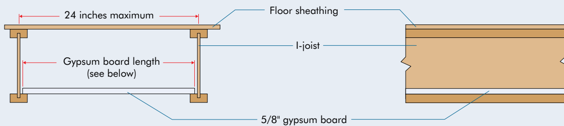
FIGURE 27 5/8-INCH GYPSUM BOARD
